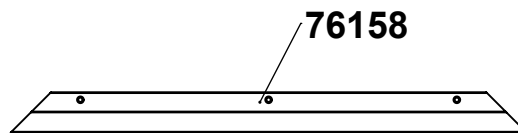
614x48x32mm
