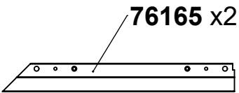
394x48x32mm
